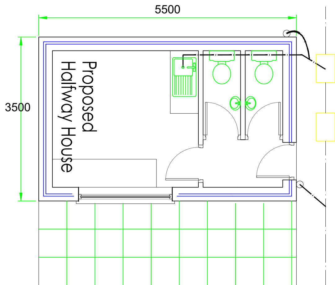
Ground Floor Plan (Scale 1:50)
